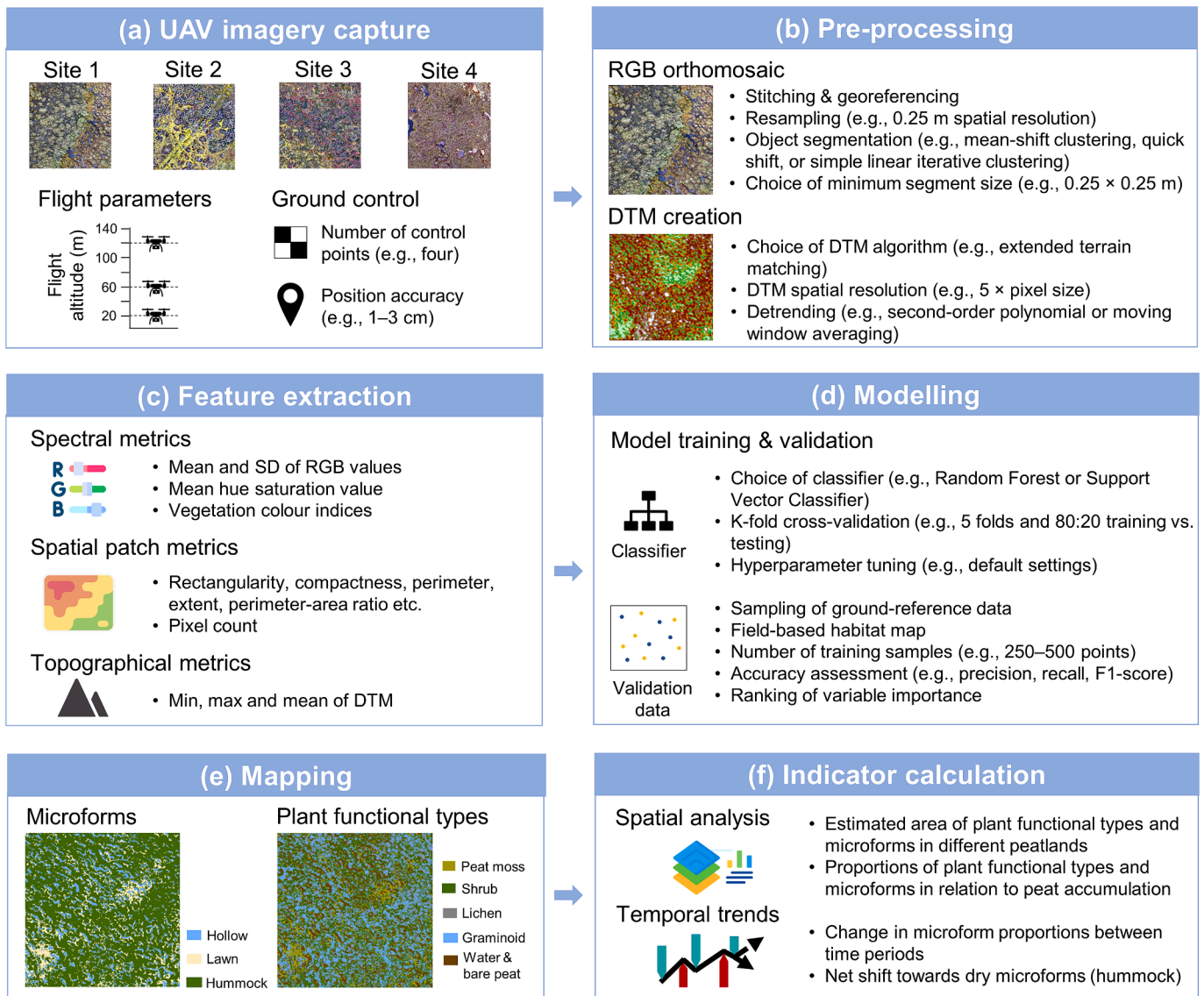
Fig. 4. Example of a workflow for processing UAV imagery into indicators of habitat condition. (a,b) Details and decisions during data collection and pre-processing, (c,d) examples of feature extraction and modelling, and (e,f) mapping of vegetation and indicator calculation. The figure synthesizes details of a workflow that has been applied to the monitoring and mapping of peatlands in Ireland (Steenvoorden et al., 2023; Steenvoorden et al., 2024; Steenvoorden and Limpens, 2023; Steenvoorden et al., 2022). These peatlands especially represent blanket bogs (Natura 2000 habitat code: 7130) and active raised bogs (Natura 2000 habitat code: 7110).
