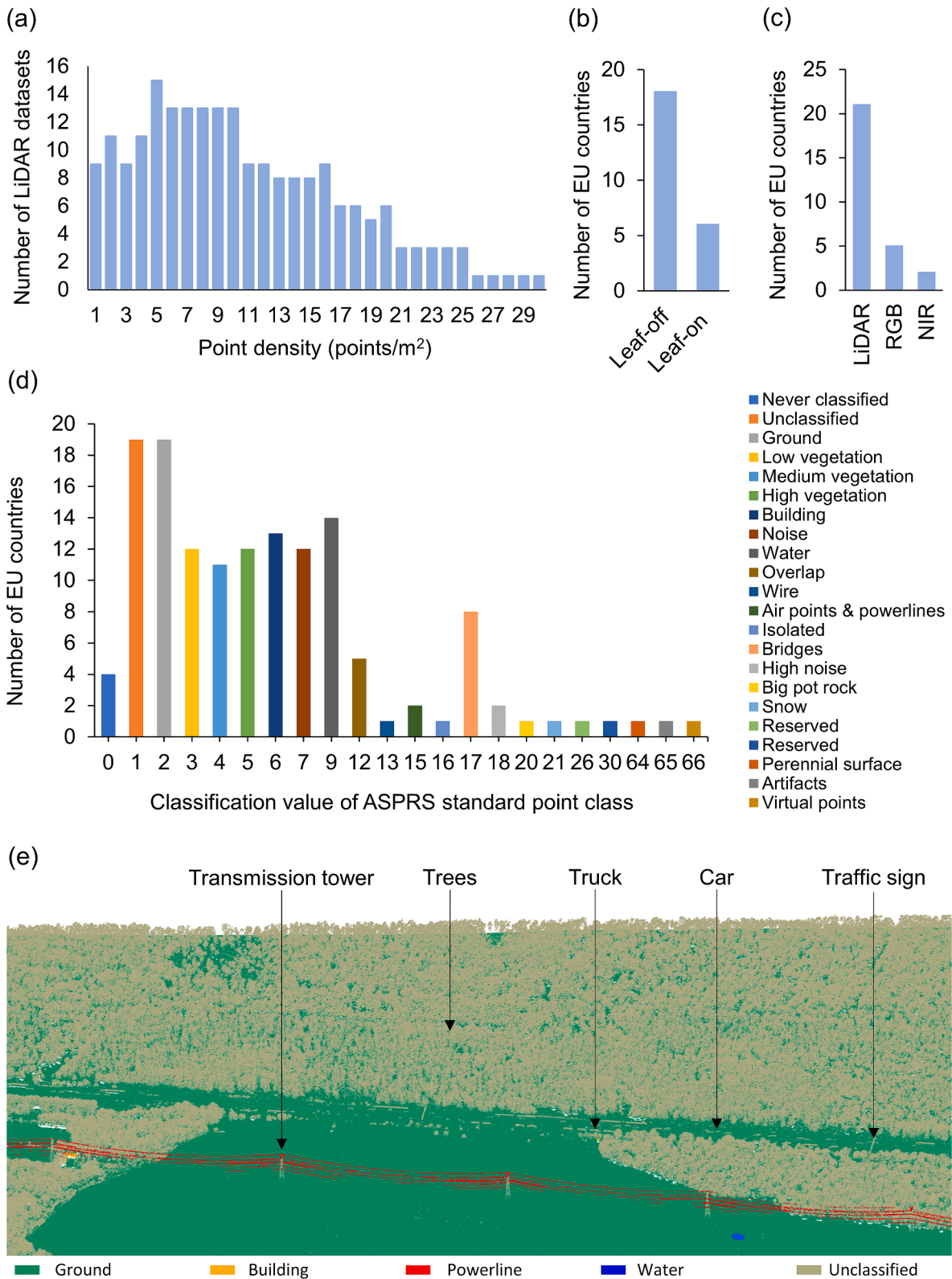
Fig. 3. Variation in characteristics of LiDAR point clouds collected through (sub)national ALS surveys in Europe (see details in Appendix A Table A1 ). (a) Range of available point densities; (b) Season of data acquisition (leaf-on vs. leaf-off); (c) Available information on LiDAR and simultaneously collected imagery in the Red, Green and Blue (RGB) and Near-Infrared (NIR) spectrum; (d) Available point classifications following the ASPRS standard point classes. (e) Example of a LiDAR point cloud (AHN4 dataset from the Netherlands) in which vegetation and non-vegetation objects (e.g., trees, transmission towers, traffic signs, trucks, and cars) are included in the same class ('unclassified', olive). The 'ground' class (green) includes ground points (i.e., terrain), but also short-stature vegetation (e.g., grasses). White areas indicate areas with no data (e.g., building fronts, below trees). The image depicts an area in the southwest of the 'De Veluwe' (Natura 2000 site code NL9801023) which is in the center of the Netherlands (52.0875278 N, 5.9507778 E). The nature reserve is mainly composed of heath and scrubs (Natura 2000 habitat code N08) and coniferous and mixed woodlands (Natura 2000 habitat codes N17 and N19), but highways and an overhead powerline are crossing.
