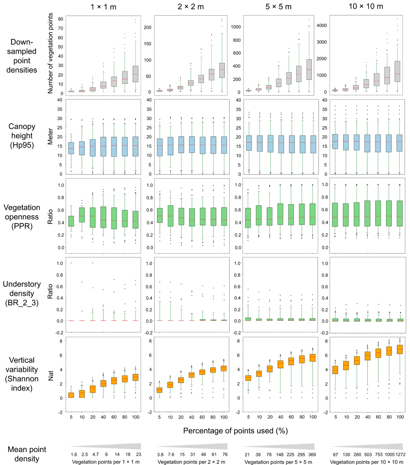
Fig. 5. The effect of grid cell spatial resolution and varying point densities on the robustness of LiDAR vegetation metrics derived from airborne ALS point clouds. LiDAR vegetation metrics were calculated at four spatial resolutions (i.e., 1 × 1 m, 2 × 2 m, 5 × 5 m and 10 × 10 m) with six systematically down-sampled point clouds (i.e., keeping 5 %, 10 %, 20 %, 40 %, 60 % and 80 % of the points from the original Dutch AHN4 dataset ‘100 %’). Mean point densities are given for each percentage of points used. Metrics were calculated using randomly located woodland plots in the Netherlands ( n = 94 ). See Appendix Fig. B4–B7 for additional metrics, and Appendix B Table B1 for metric abbreviations and definitions.
